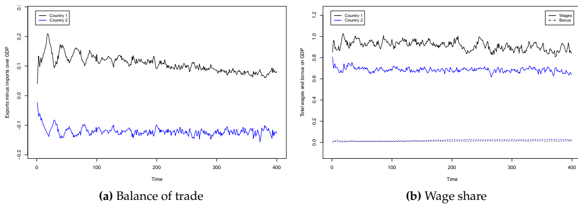
Figure 8: Country performance in trade and wages as share of GDP. Time-series medians from 50 Monte Carlo runs, excluding warm-up period. Country colour: North (1) black, South (2) blue.
