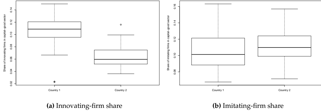
Figure 9: Country share of innovating and imitating firms in capital-good sector. Distributions from 50 Monte Carlo runs, t \in [201 - 400] . Bar: medians, box: 2nd/3rd quartiles, whiskers: minimum/maximum, points: outliers. Country number: North (1), South (2).
