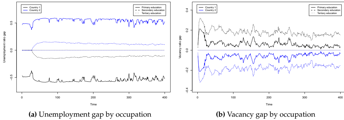
Figure 7: Country gaps in unemployment and vacancy. Time-series medians from 50 Monte Carlo runs, excluding warm-up period. Country colour: North (1) black, South (2) blue.
