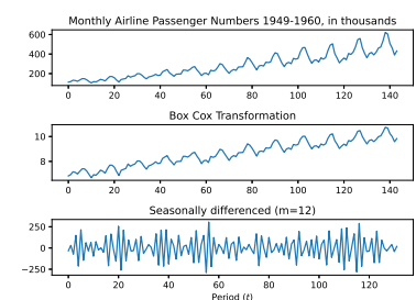
Fig. 83 Airline time series: Box-Cox transformation and seasonal differencing.
