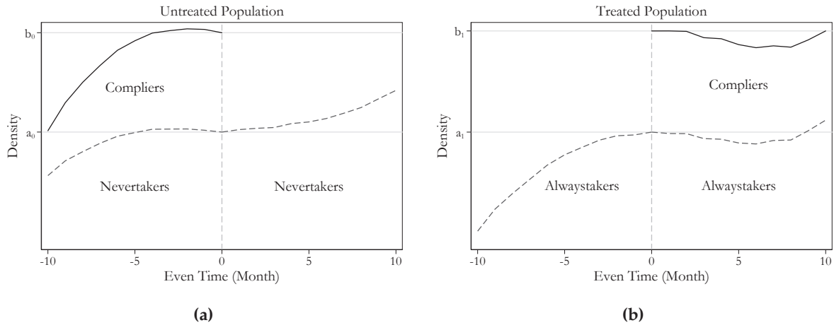
Figure 8: Selection Analysis.
