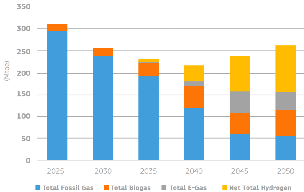
Figure 1: Fit for 55 forecast consumption of gaseous fuels
