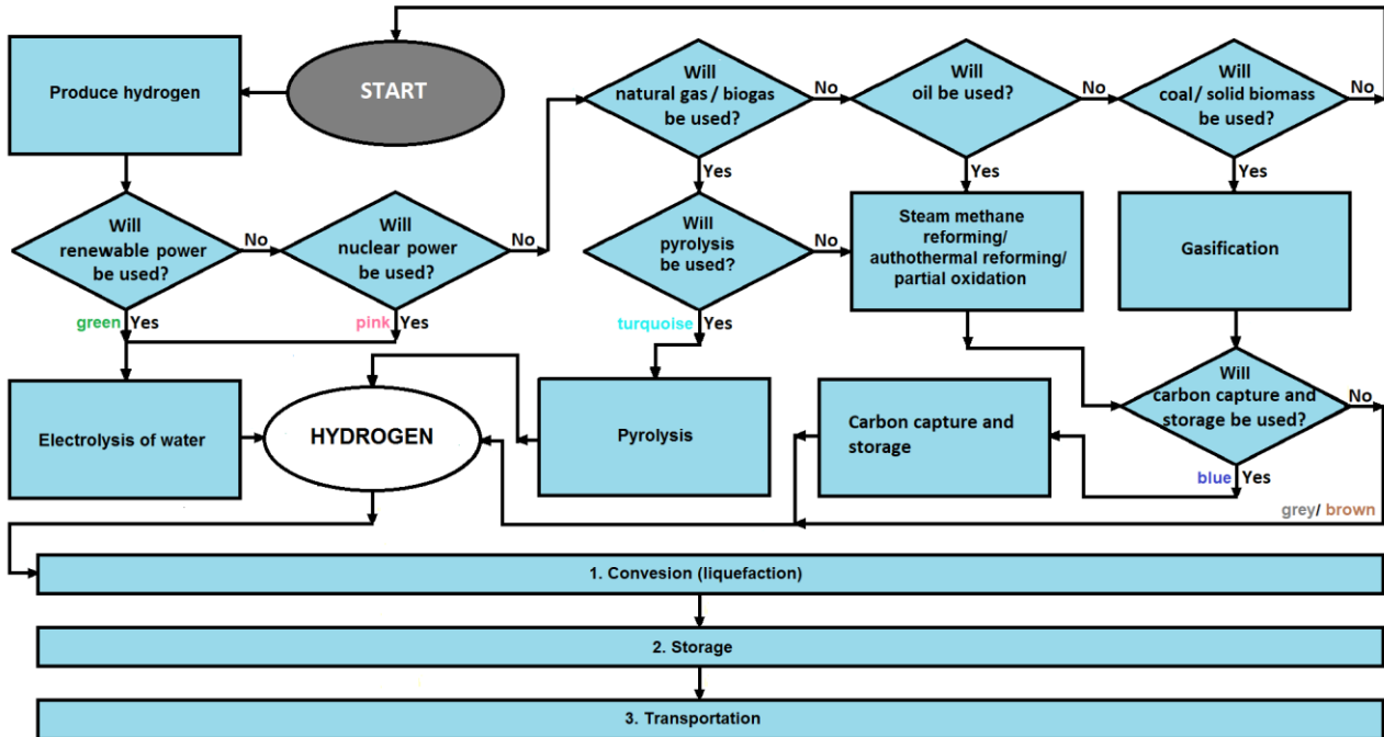
Figure 2: Simplified decision-making and value chain flow chart for the large-scale production of most common ‘colours’ of hydrogen
