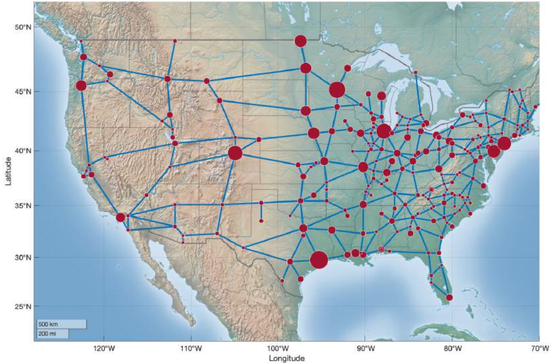
Figure 10. Welfare Gains
