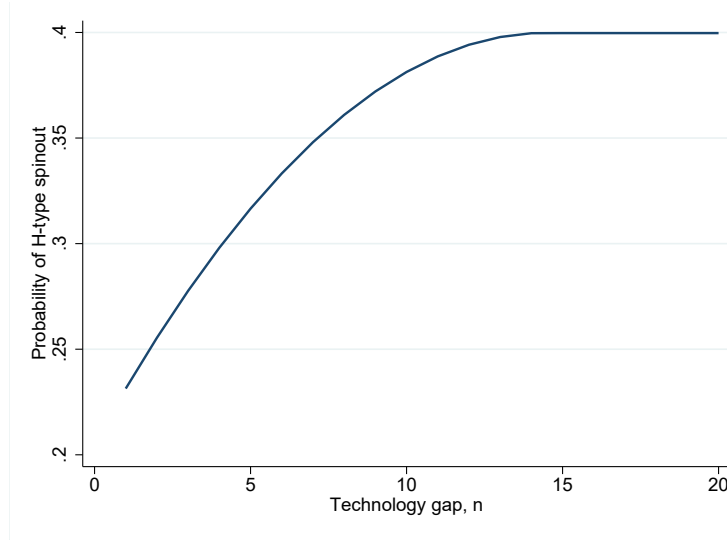
Figure 4: Calibration: \mu_n estimates
