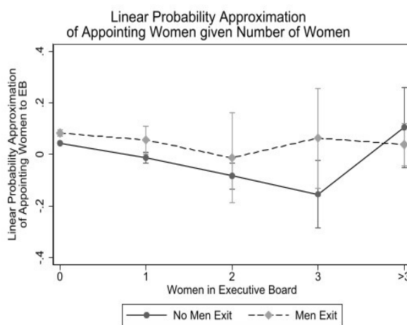
(a) TABLE 5 SPECIFICATION (4) WITH MEN EXIT INTERACTION
