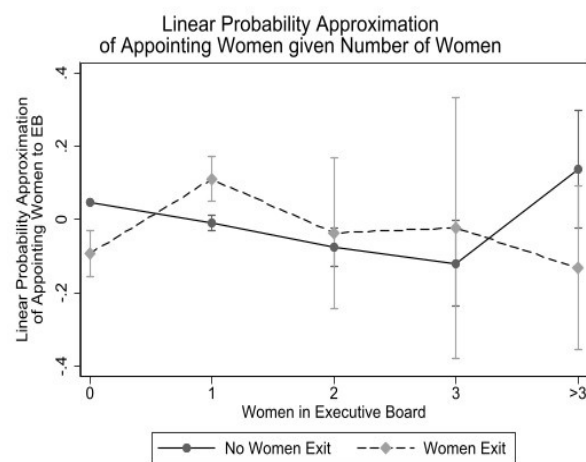
(b) TABLE 5 SPECIFICATION (4) WITH WOMEN EXIT INTERACTION
