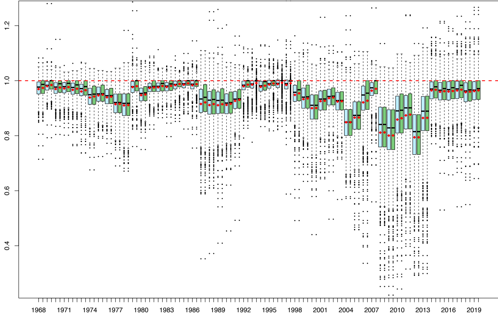
Figure 8: Five-factor-model boxplots for the two ratios defined in (4.1) for large-cap stocks. For any year, we plot first the WLS/OLS boxplots in blue, followed by the ALS/OLS boxplots in green. In each box, the bar indicates the median ratio whereas the diamond-shaped symbol indicates the average ratio.
