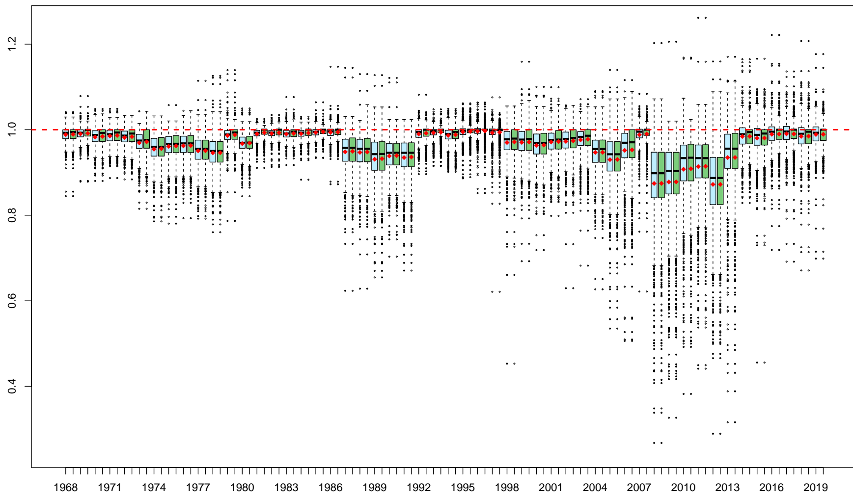
Figure 4: Similar to Figure 2 except that we now restrict attention to large-cap stocks.
