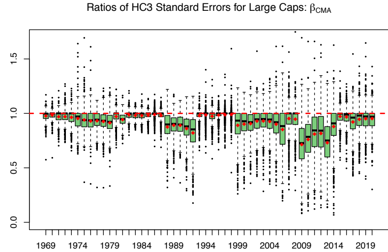
Figure 10: Five-factor-model boxplots for the SMB, HML, RMW and CMA \beta 's ratios defined in (4.1) for large-cap stocks. Due to readability we plot only the ALS/OLS boxplots in green. However, in unreported results we find similar patterns for WLS/OLS.
