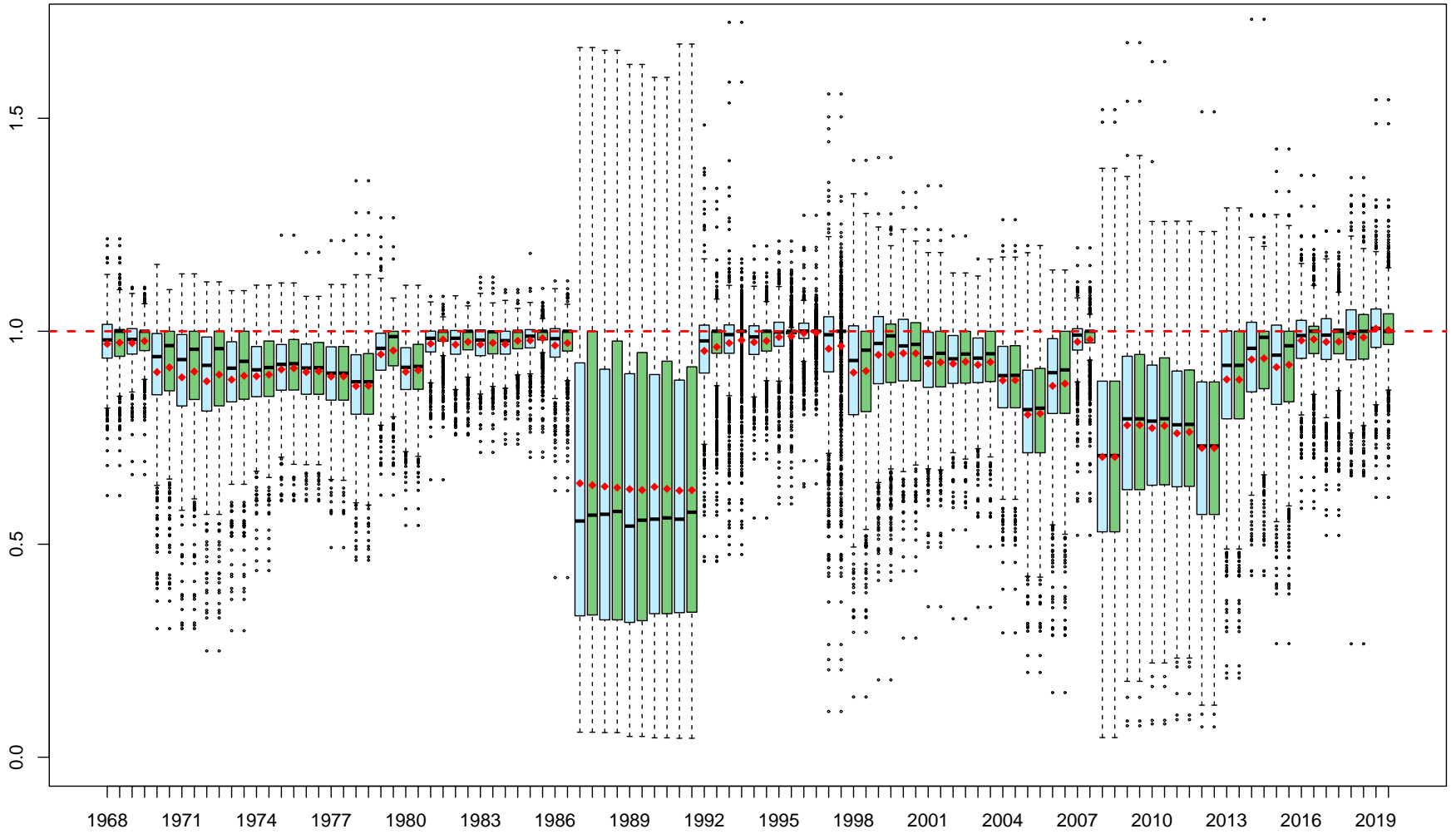
Figure 5: Similar to Figure 3 except that we now restrict attention to large-cap stocks.
