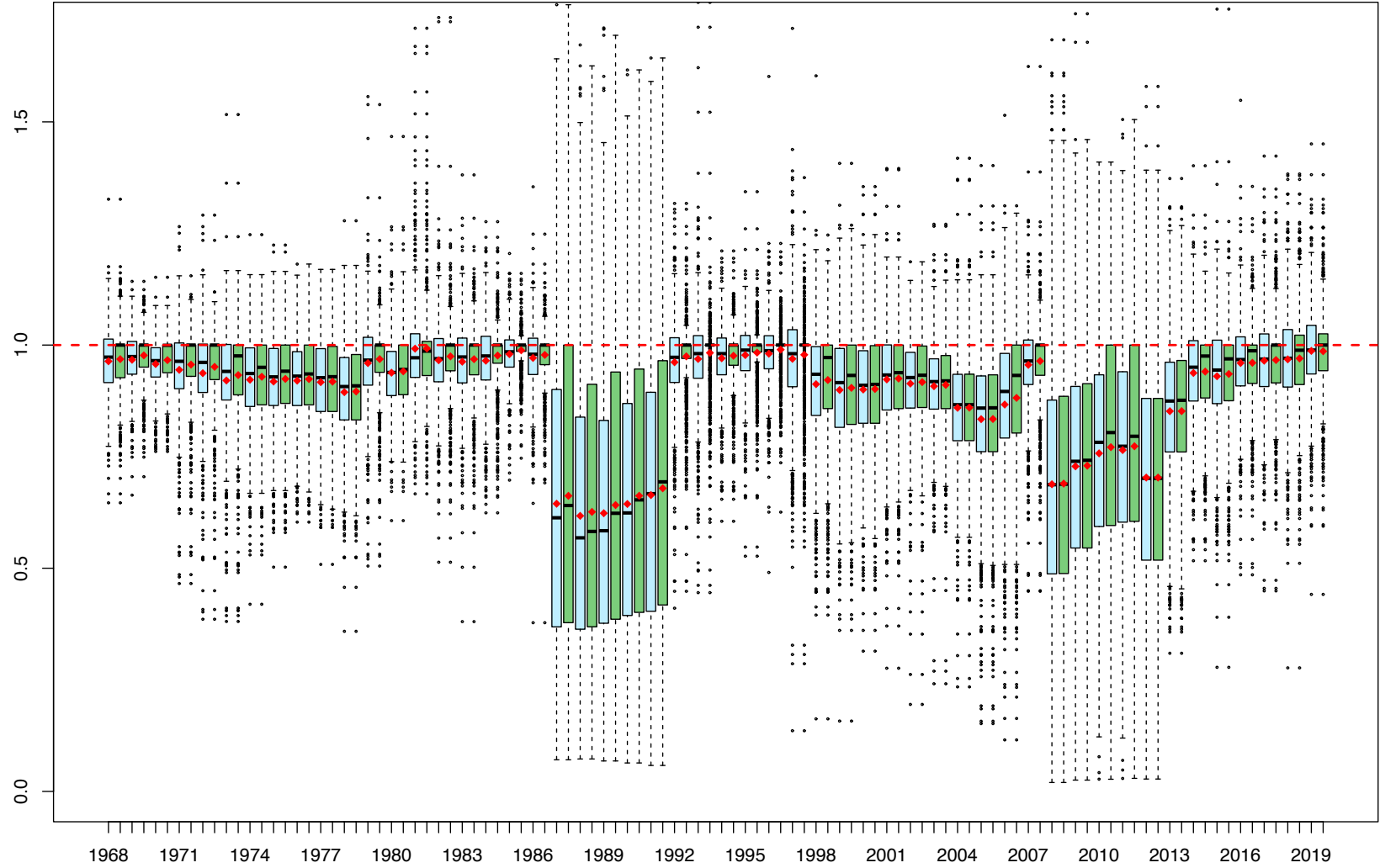
Figure 9: Five-factor-model boxplots for the market factor \beta ratios defined in (4.1) for large-cap stocks. For any year, we plot first the WLS/OLS boxplots in blue, followed by the ALS/OLS boxplots in green. In each box, the bar indicates the median ratio whereas the diamond-shaped symbol indicates the average ratio.
