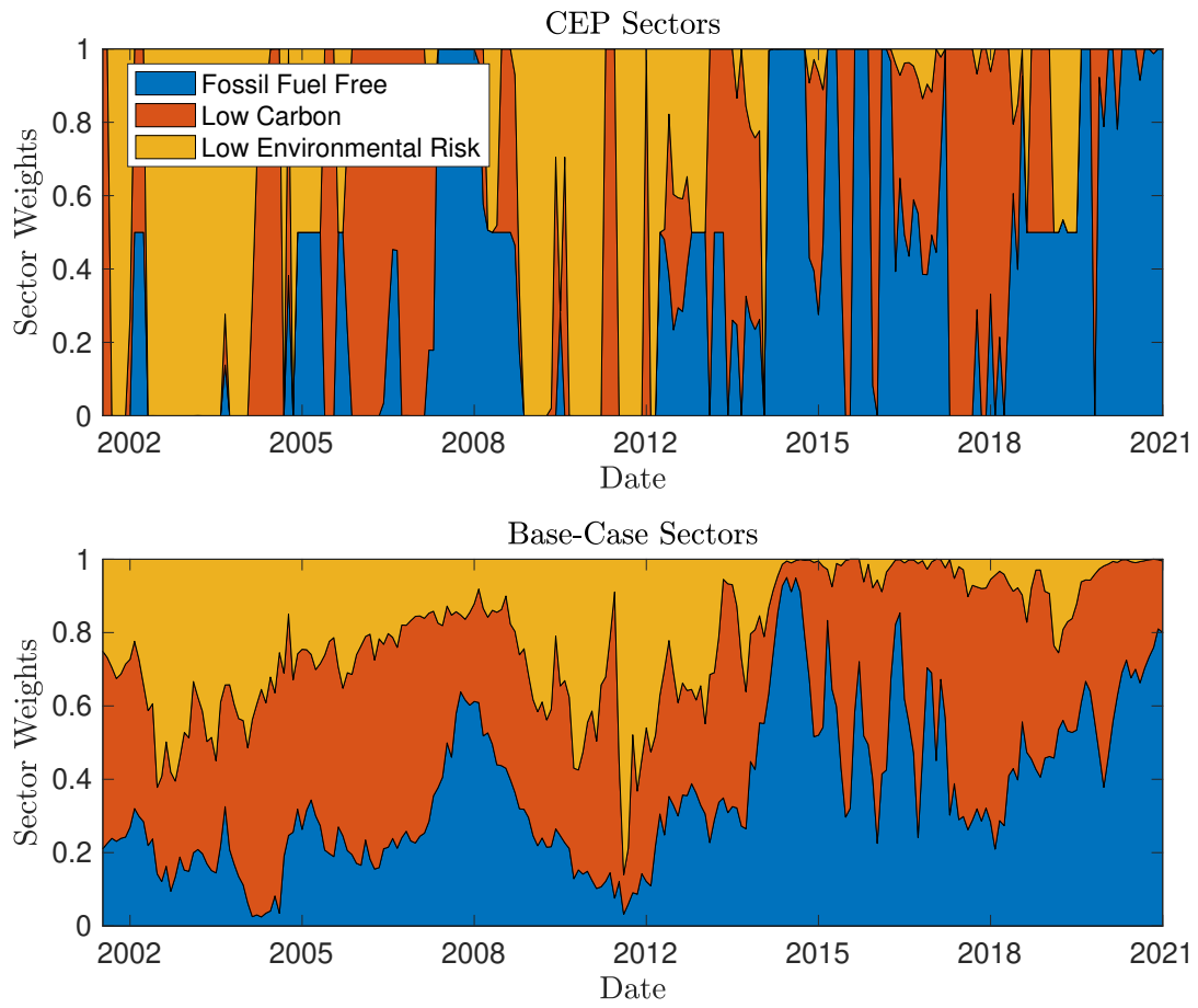
Figure 8: The panel on the top shows the sector weights of the CEP ( \lambda = 0.0022 ) and the panel on the bottom shows the sector weights of the base case over time.
