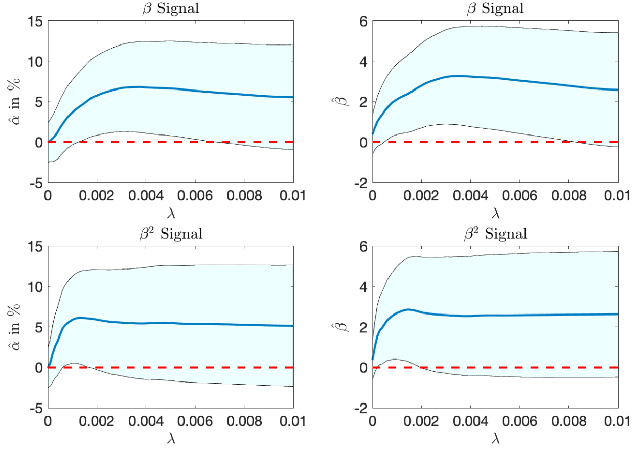
Figure 9: Shows the (annualized) \hat{\alpha} and \hat{\beta} , and their 95% confidence interval based on HC3 standard errors, for various efficient factor mimicking portfolios of the NYT climate news based on the \beta and \beta^2 signal.
