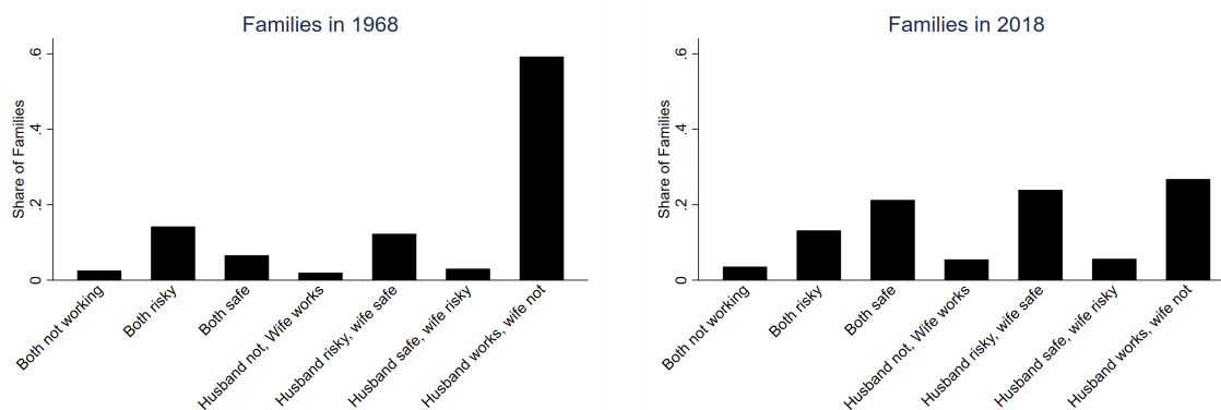
Figure 23.: Family types
