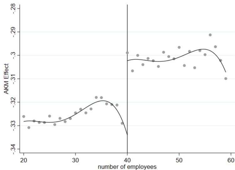
AKM Firm Fixed Effects
