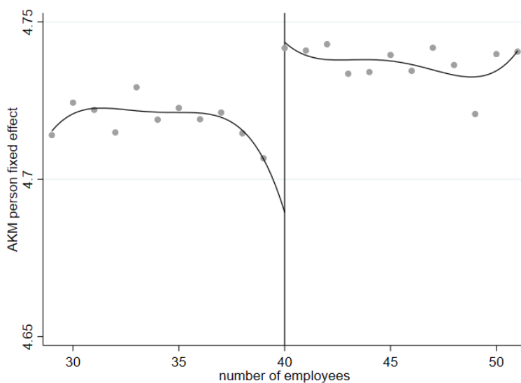
AKM Person Fixed Effects
