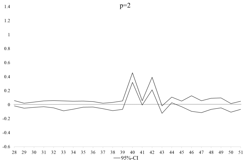
Figure B.12: Placebo Thresholds (Polynomial Order 2)
