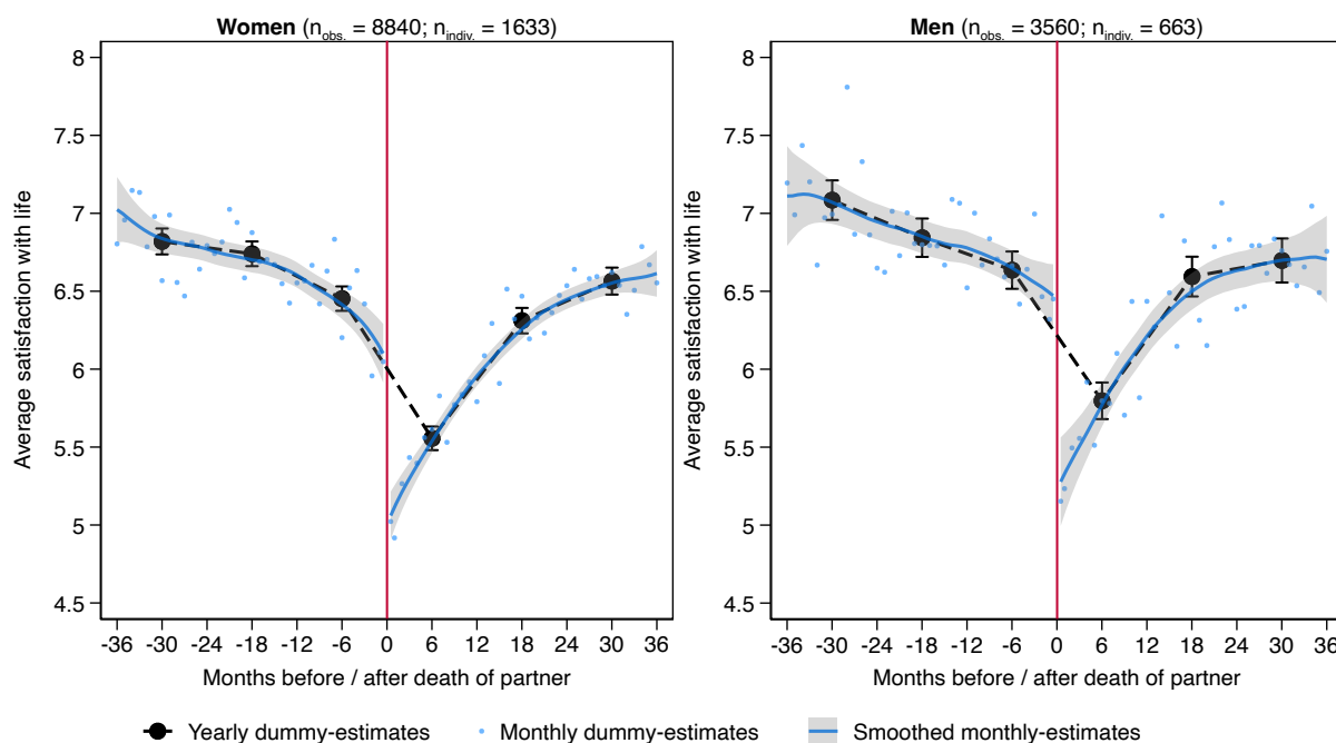
Figure 5. Overall life satisfaction around the time of the death of a partner, based on SOEP data. A comparison of yearly dummy estimates, monthly dummy estimates, and smoothed monthly estimates.
