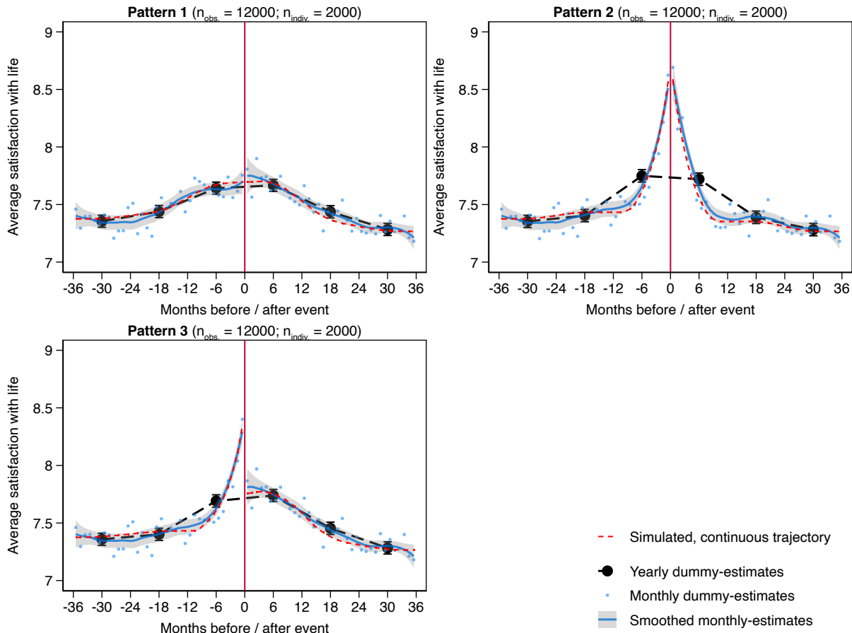
Figure 1. Simulation analyses, a visual comparison of three analytical approaches: yearly dummy estimates, monthly dummy estimates, and smoothed monthly estimates.
