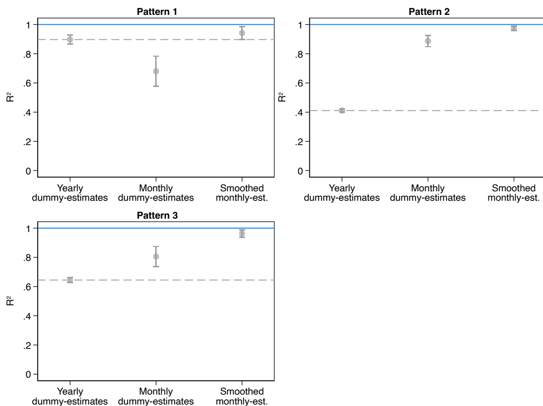
Figure 2. Simulation analyses, statistical comparison of three analytical approaches: yearly dummy estimates, monthly dummy estimates, and smoothed monthly estimates; based on 1,000 iterations of the simulation process.
