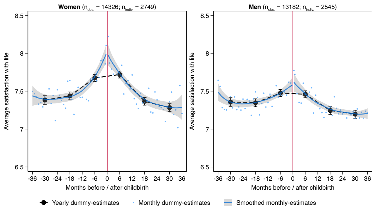
Figure 4. Overall life satisfaction over the transition to parenthood, based on SOEP data. Comparison of yearly dummy estimates, monthly dummy estimates, and smoothed monthly estimates.
