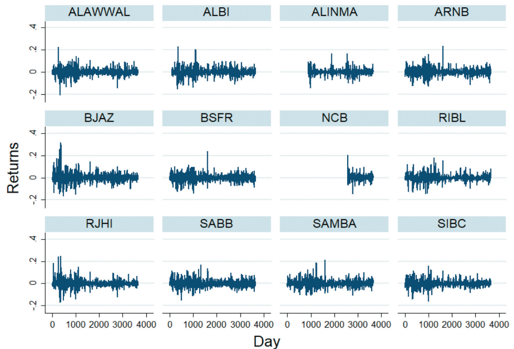
Figure 4. The daily returns of Saudi banks stocks from 3/1/2005 to 31/12/2018.
