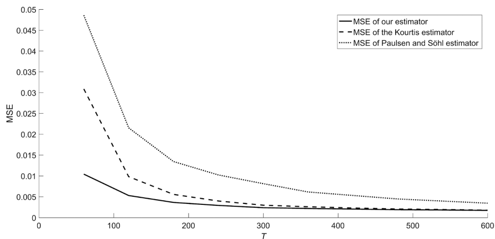
Figure 3. MSE of the expected Sharpe ratio estimators as a function of the estimation length.
