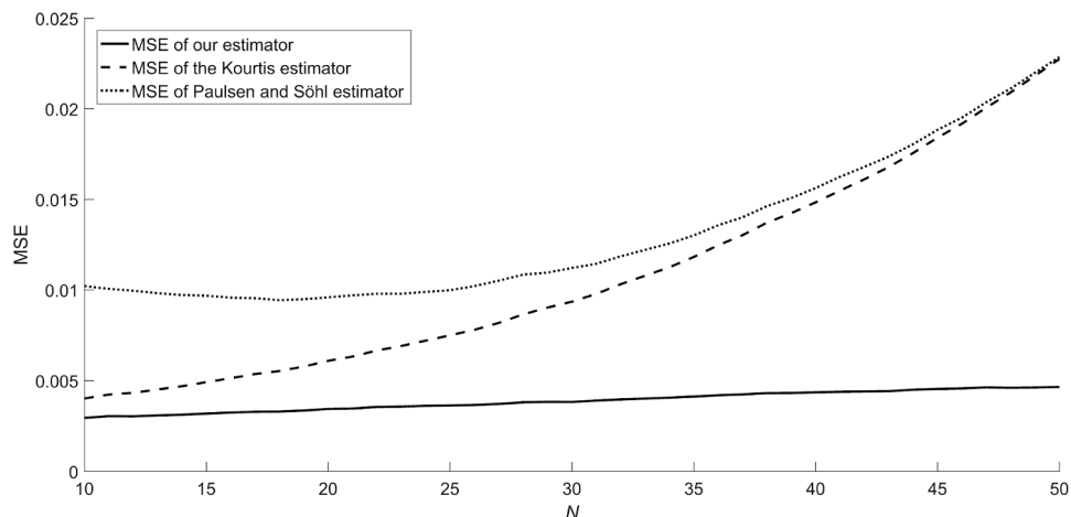
Figure 2. MSE of the expected Sharpe ratio estimators as a function of the portfolio dimension.
