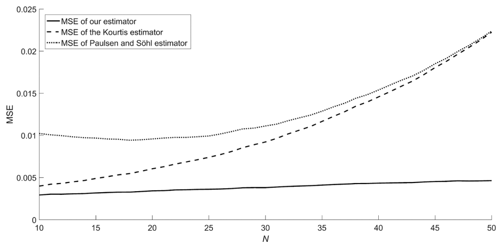
Figure 4. MSE of the expected Sharpe ratio estimators as a function of the portfolio dimension.
