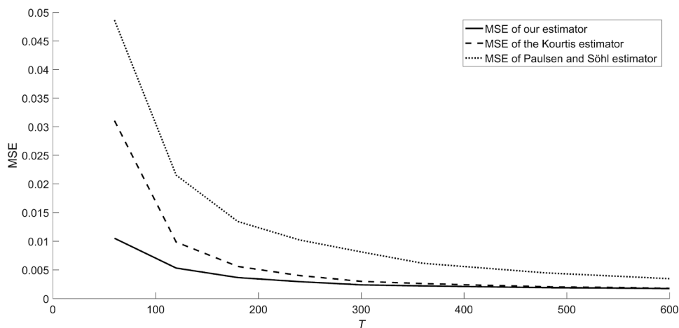
Figure 1. MSE of the expected Sharpe ratio estimators as a function of the estimation length.
