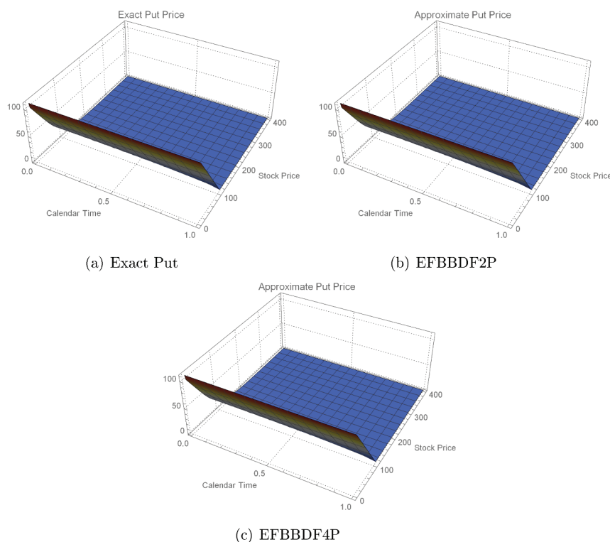
Figure 7. The values of the put option as a function of stock price and time computed using the EFBBDF2 and EFBBDF4 for M = 200 and N = 12 . Exact Solution is included for comparison. The value of the put at the stock price of s = 100 is $17.98.
