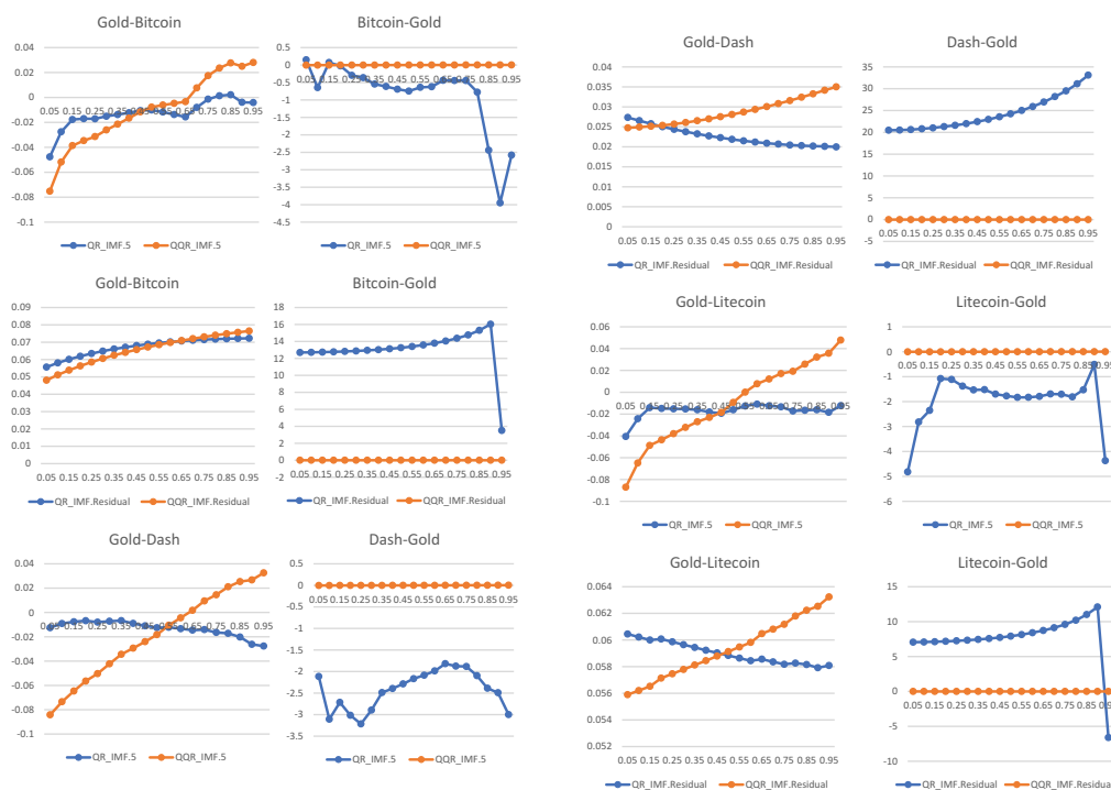
Figure 2. Bi-directional gold and cryptos QR and QQR.
