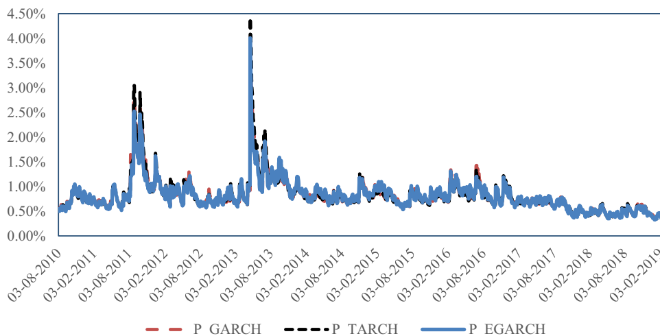
Figure 3. Price Volatility of 50 Baht Gold Futures predicted using GARCH Family Models.
