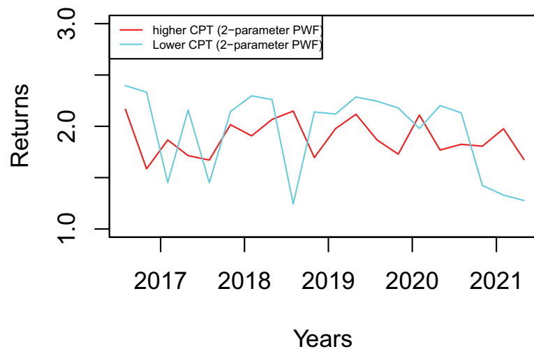
Figure 6. Indices returns comparison (2-parameter PWF).
