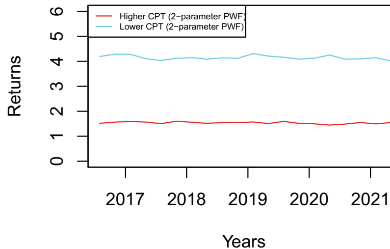
Figure 7. Mixed assets returns comparison (2-parameter PWF).
