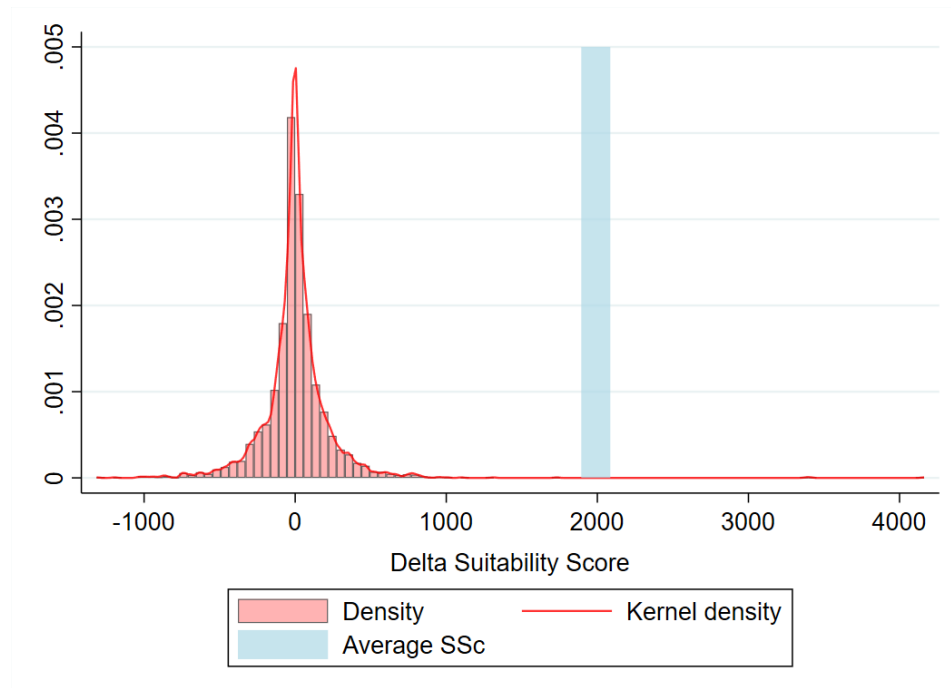
Figure 6: Distribution of the variation in Suitability Score between 2000 and 2010
