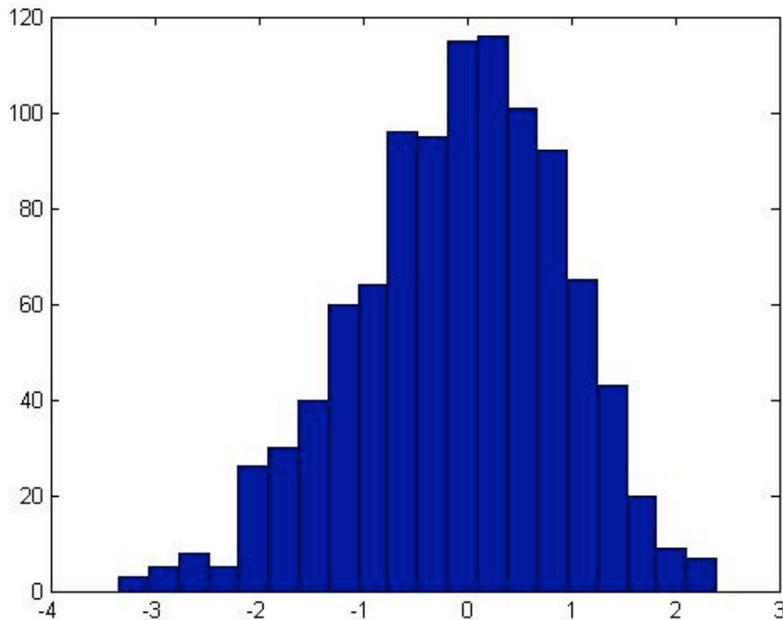
FIGURE 2. Bootstrapped histogram
