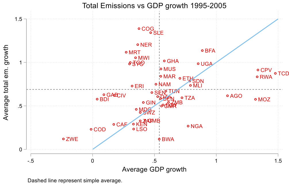
Figure 3: Decadal growth rates: CO2e emissions vs. GDP across Africa
