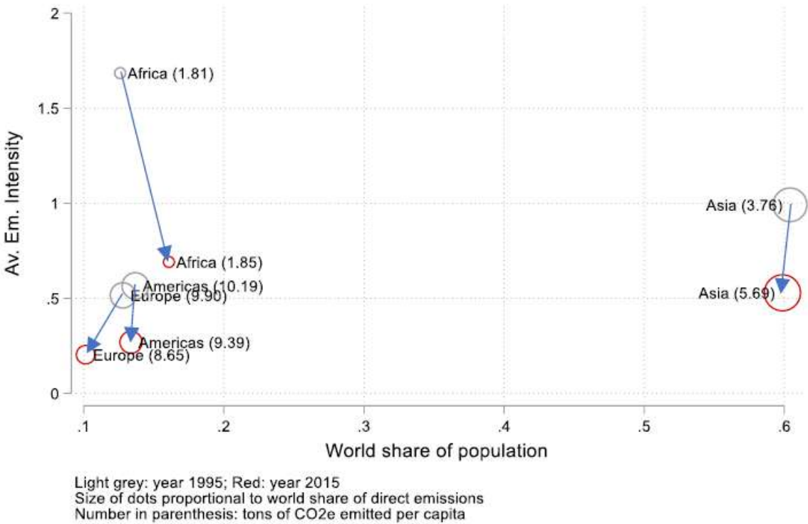
Figure 1: CO 2 e emissions, population shares, and per capita emissions by region: 1995 and 2015
