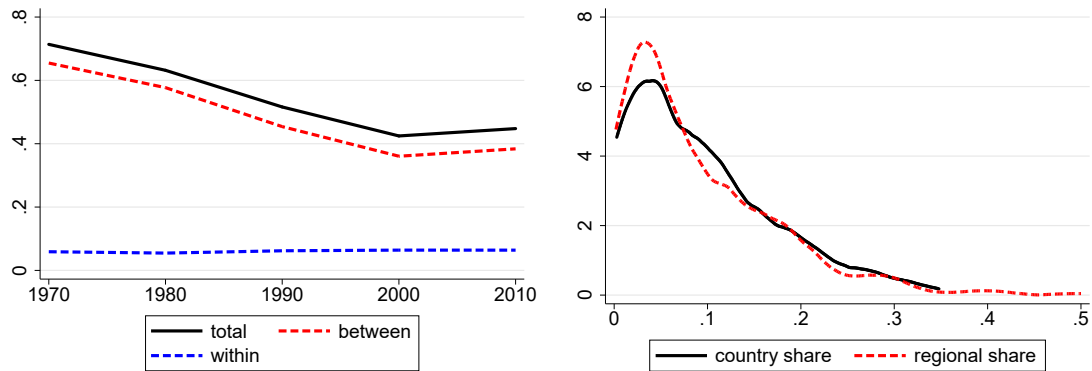
(a) Theil indices of inequality in the share of college graduates 1970-2010 (b) Kernel density of the share of college graduates in 2010
