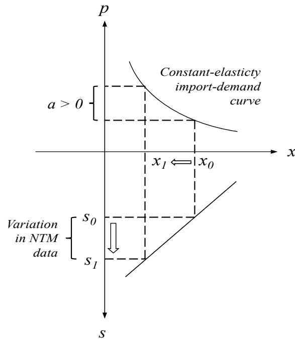
Figure 1: AVE determination in the absence of market failure
