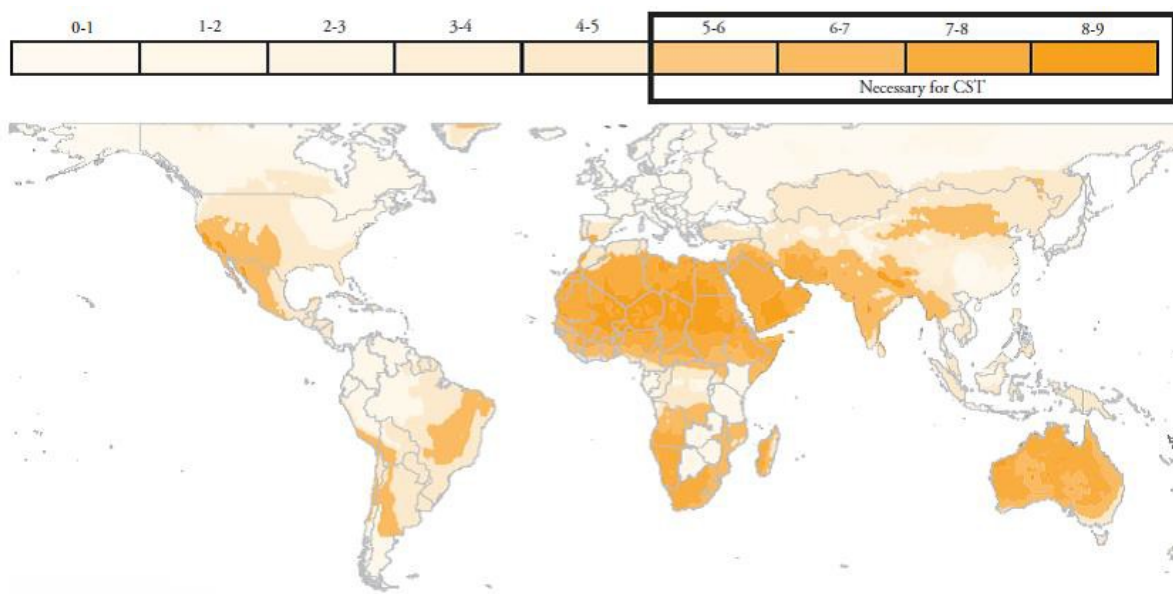
Fig. 1: Africa has a clear advantage in solar based on its irradiation potential (Global Direct Normal Solar Radiation (kW/m 2 /day))
