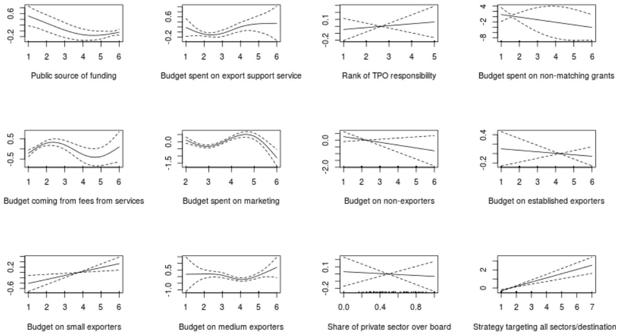
Figure 6: First stage regression explaining EPAs' budgets
