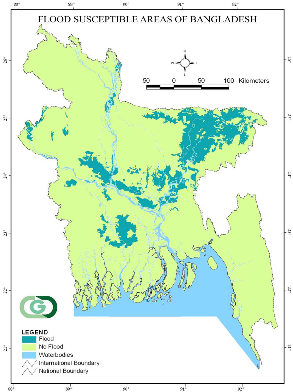
Figure 2: Flood susceptible areas of Bangladesh
