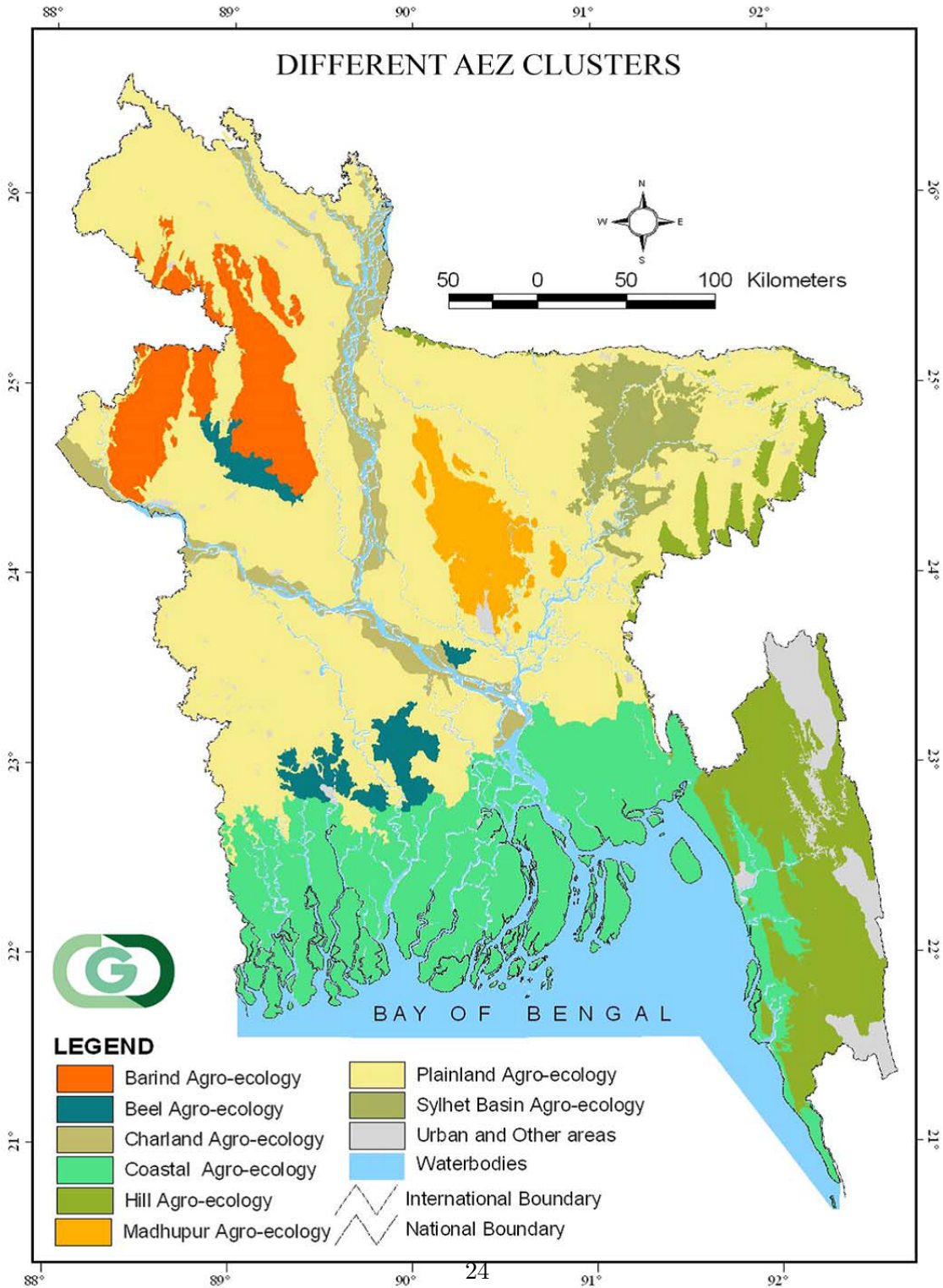
Figure 1: Differences in AEZ
