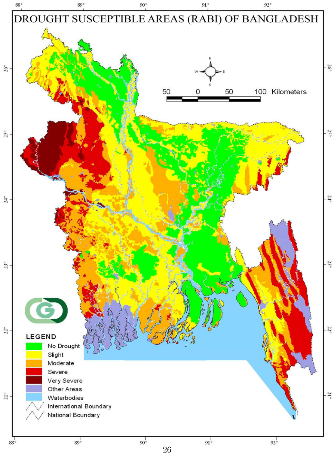
Figure 3: Drought susceptible areas of Bangladesh
