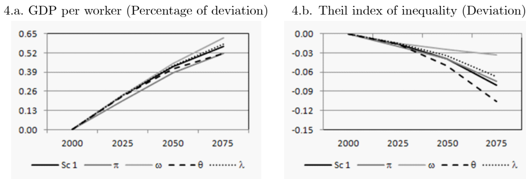
Figure 4. Robustness analysis
