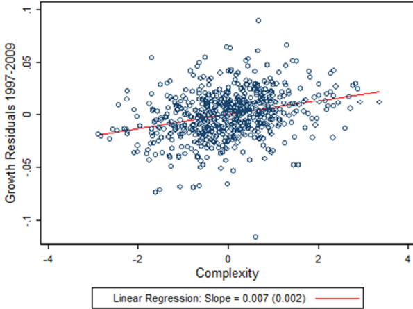
(a) Complexity
