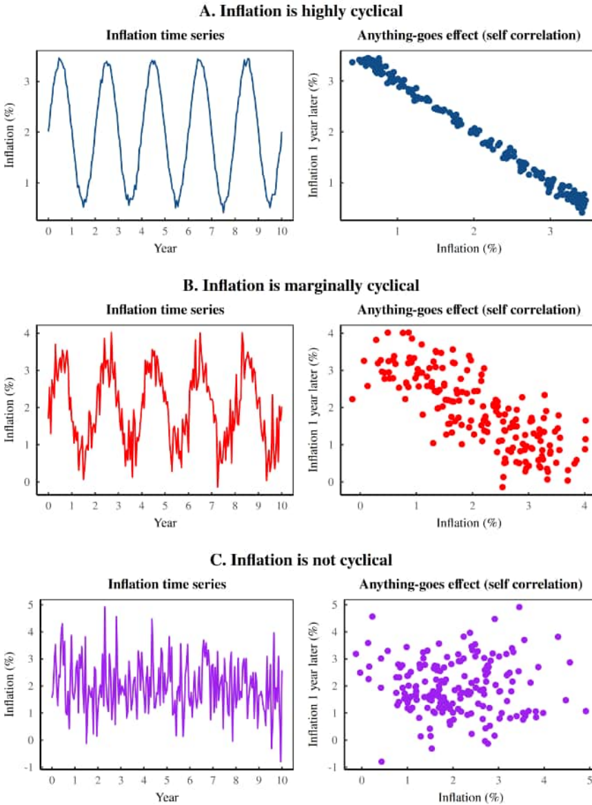
Figure 8: Measuring self correlation — the ‘anything-goes’ effect
