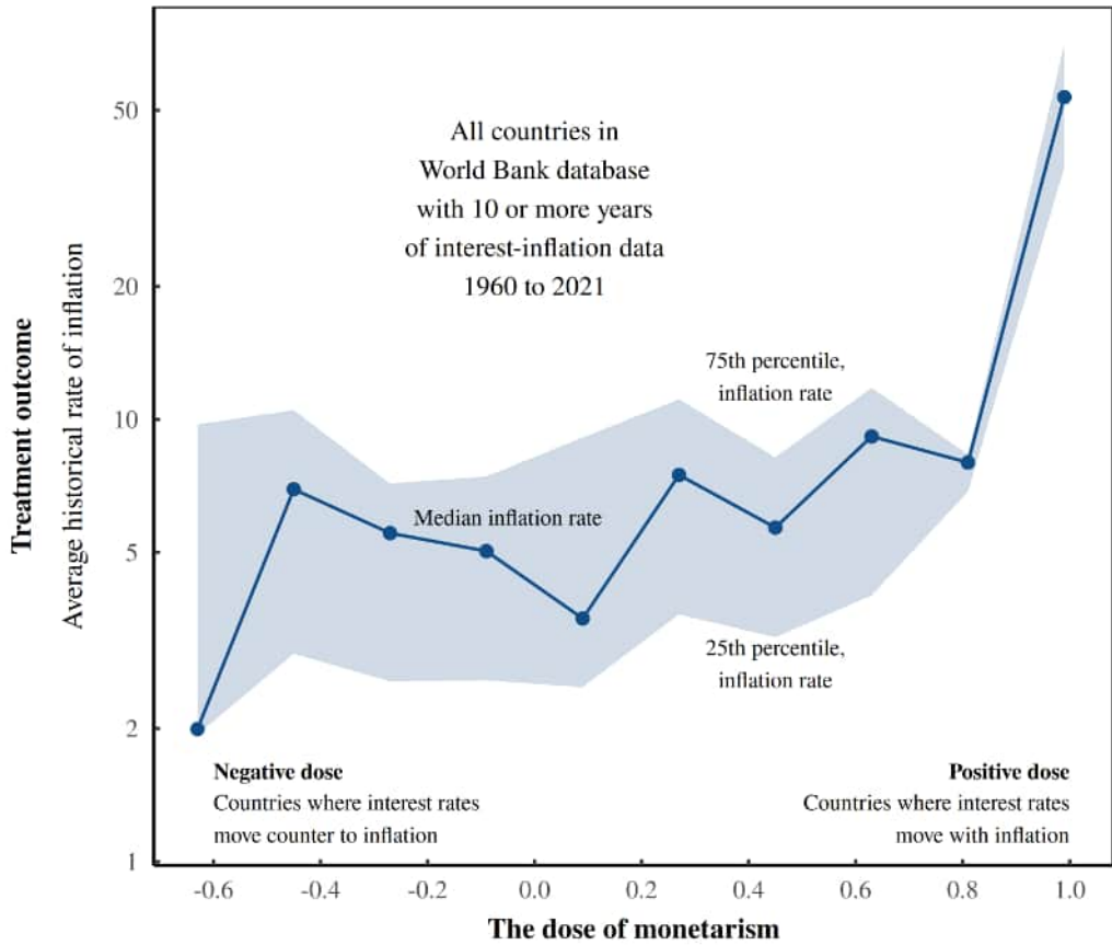
National correlation between annual interest-rate change and inflation rate change
