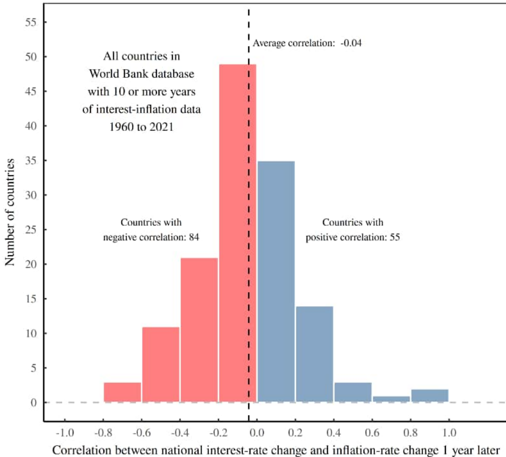
Figure 7: Change in interest rates precede changes in inflation — the correlation within countries
