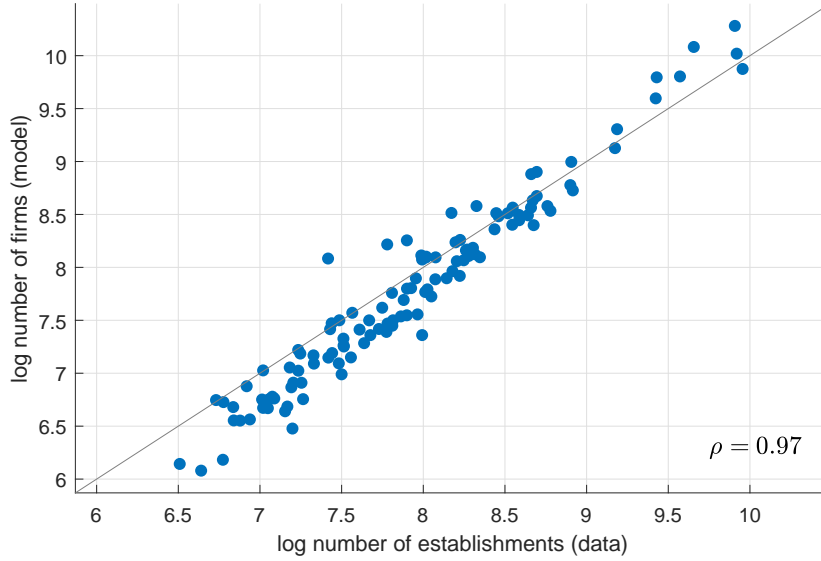
Figure 3: Predicted number of firms
