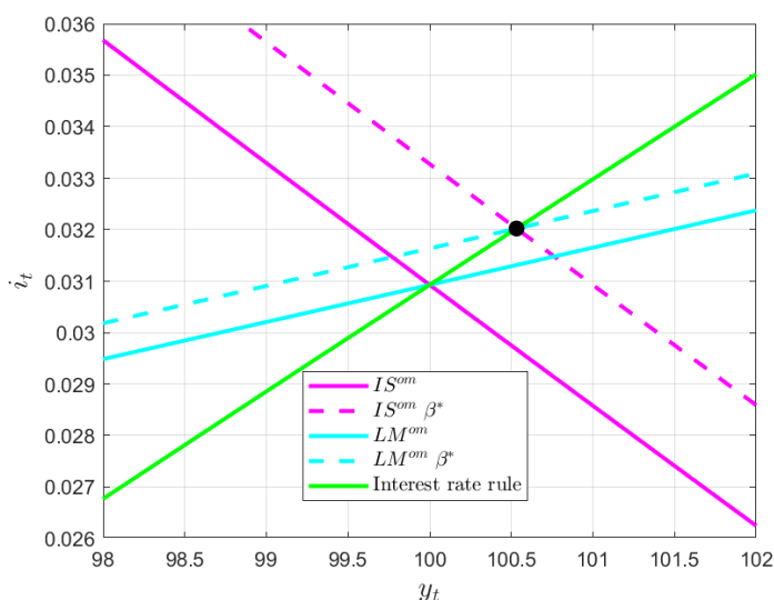
Figure 11 Households' discount factor shock in the outside-money version of the model
