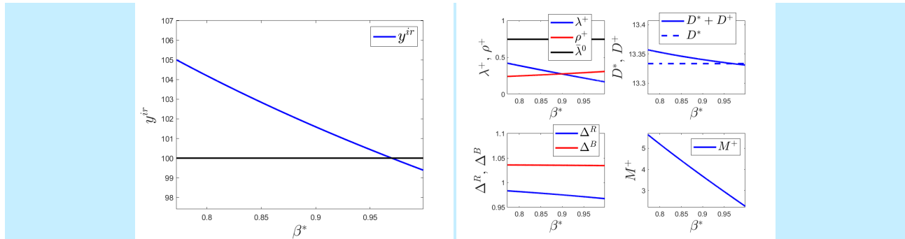
Figure 12 Implementation of the interest rate rule – households' discount factor shock
