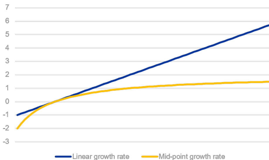
Figure A.1: Comparison between linear and mid-point growth rate
