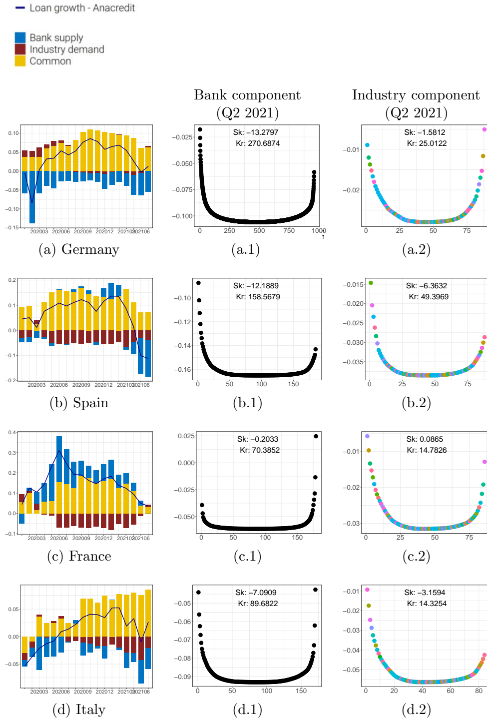
Figure 2: Credit growth decomposition and distribution of the idiosyncratic components
