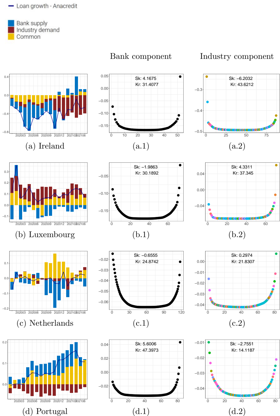
Figure C.2: Credit growth decomposition and distribution of the idiosyncratic components
