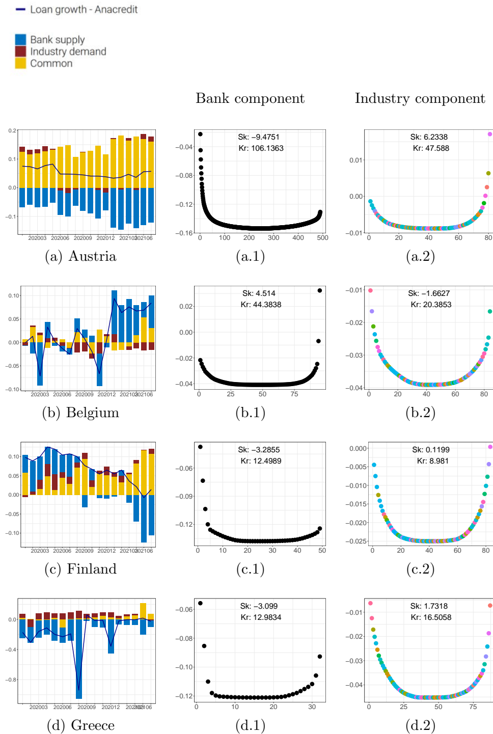
Figure C.1: Credit growth decomposition and distribution of the idiosyncratic components
