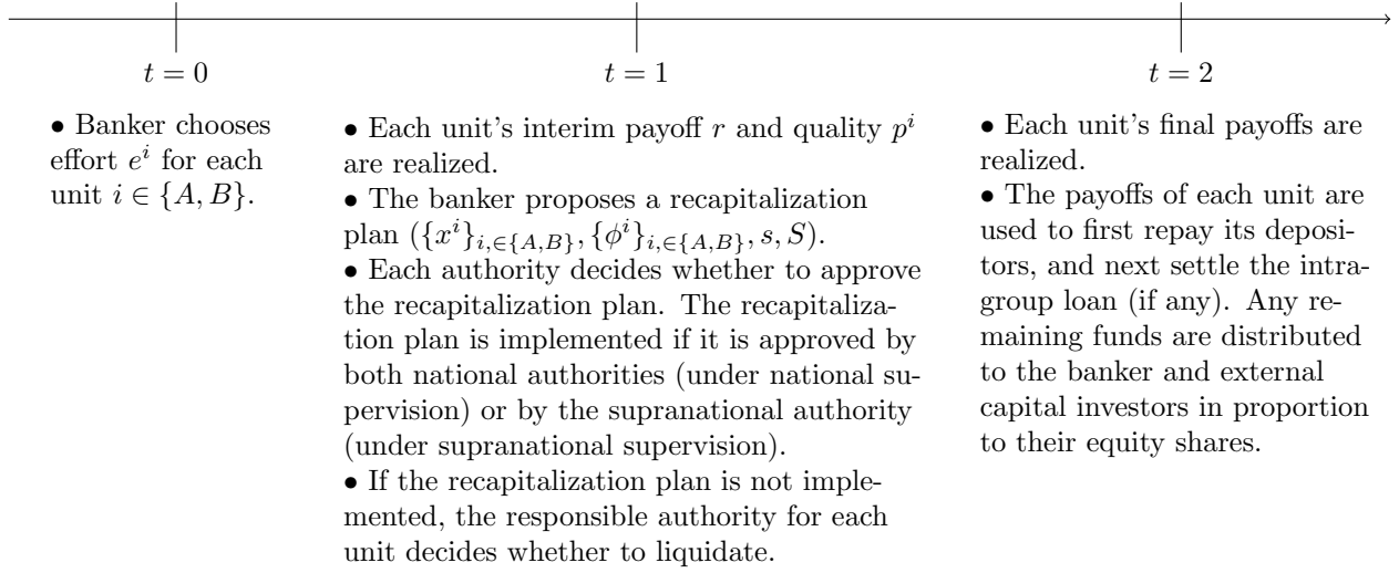
Figure 3: Time line.
