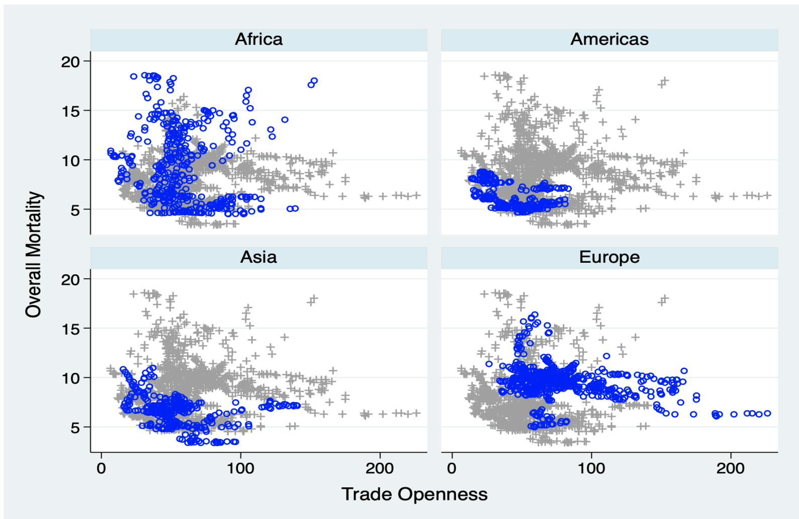
Appendix 3: Scatter plot between overall mortality and trade openness
