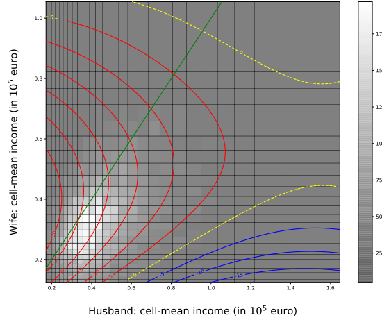
Figure 5: Supermodular core, surface levels, married in 2014, 2011 incomes
