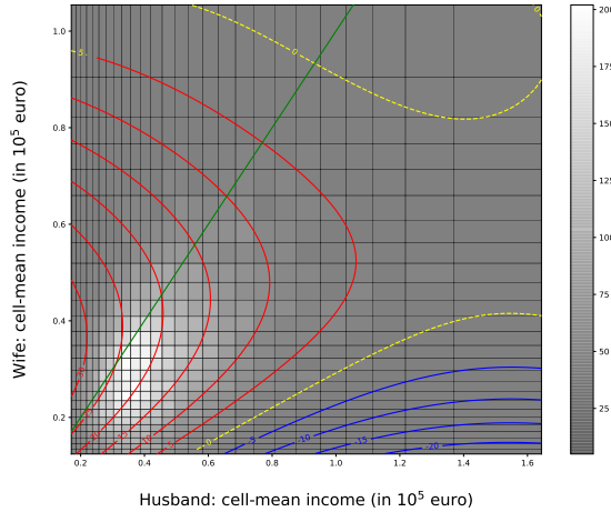
Figure 9: Supermodular core, surface levels, married 2013, average incomes
