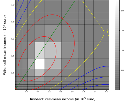
(c) Changing the discretization of the bottom 99%, using the q_{25}^z, q_{99}^z quantile range.
