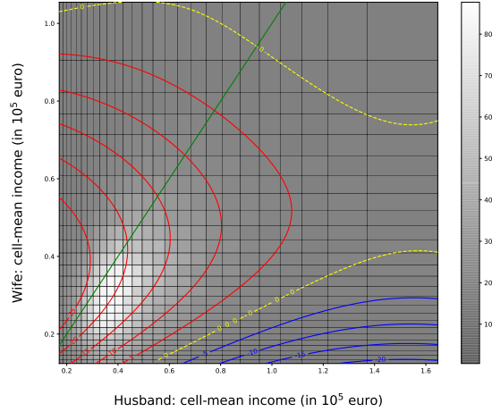
Figure 3: Supermodular core, surface levels, all newly wed
