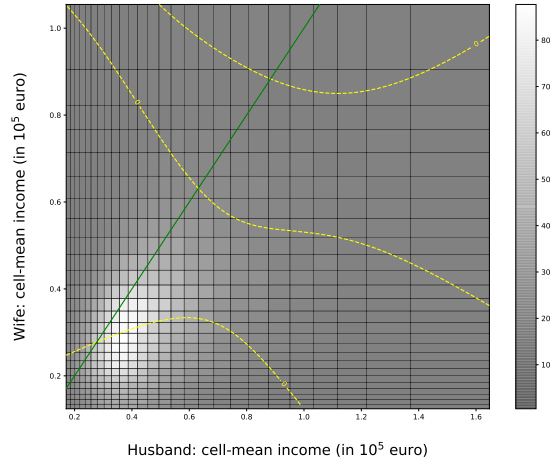
Figure 8: Placebo regression, all newly wed
