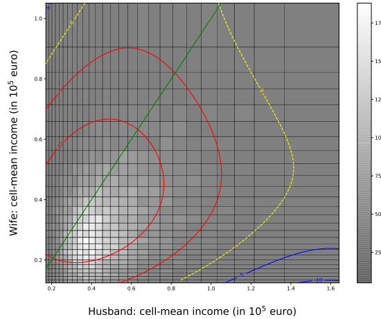
Figure 6: Supermodular core, surface levels, married 2011, 2014 incomes
