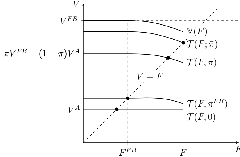
Figure 2: Determination of the fixed point of \mathcal{T}(F; \pi) = \pi \mathbb{V}(F) + (1 - \pi)V^A for different values of \pi . Drawn for \beta > \beta^{FB} and assuming \mathbb{V}(\bar{F}) > \bar{F} ; if \beta < \beta^{FB} , then F^{FB} < V^A .
