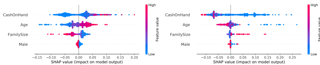
Figure A.18: SHAP values of XGBoost analysis for Italy. The left graph shows a classification on low MPC values (< 35), the right graph shows a classification on high MPC values (> 65). All data is taken from the third wave (2017) of the HFCS (HFCN, 2020b).
