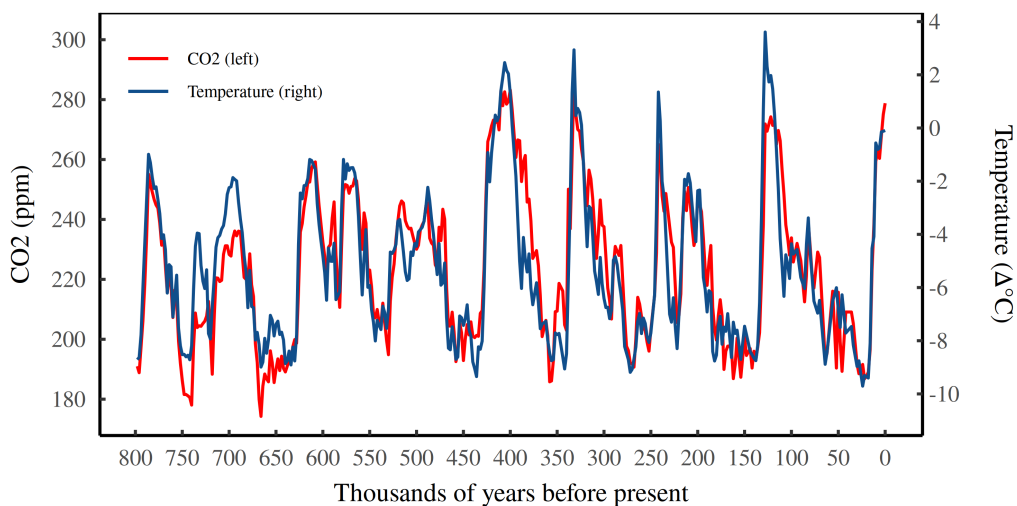
Figure 2: Carbon dioxide up-regulates the Earth’s temperature
