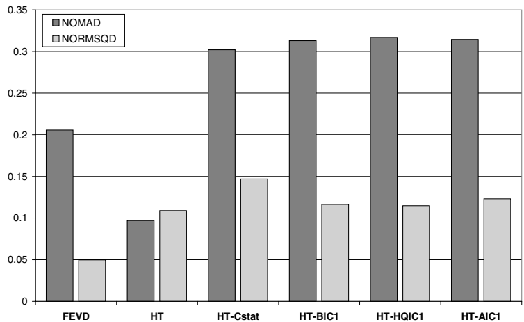
Figure 11: NOMAD and NORMSQD values averaged over all MC simulations
