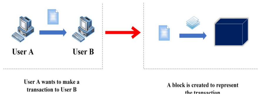
Figure 1. Blockchain process.
