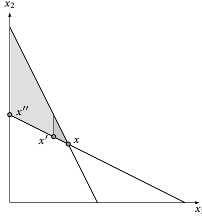
Figure 2: Both \{x', x\} and \{x'', x\} lead to the same Afriat efficiency index of 1 - \varepsilon , but have different volume violation indices.
