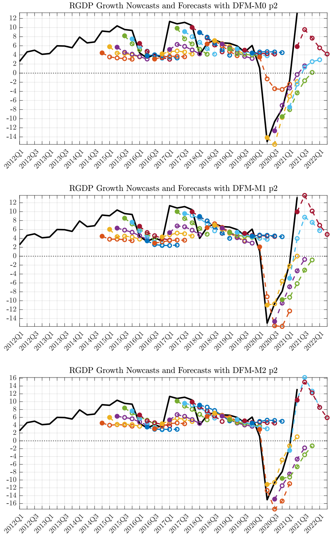
Figure 5: DFM-M p2 - Real GDP growth forecasts and nowcasts over time
