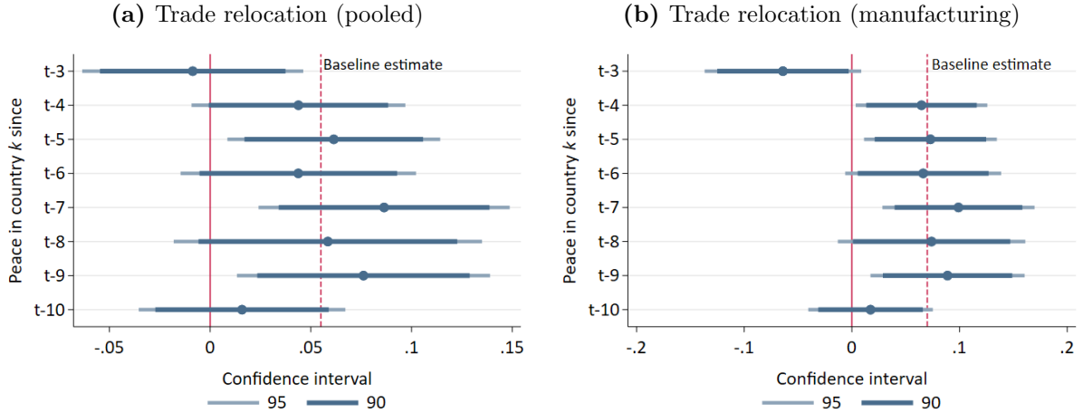
Figure 2 – Relocation persistence
