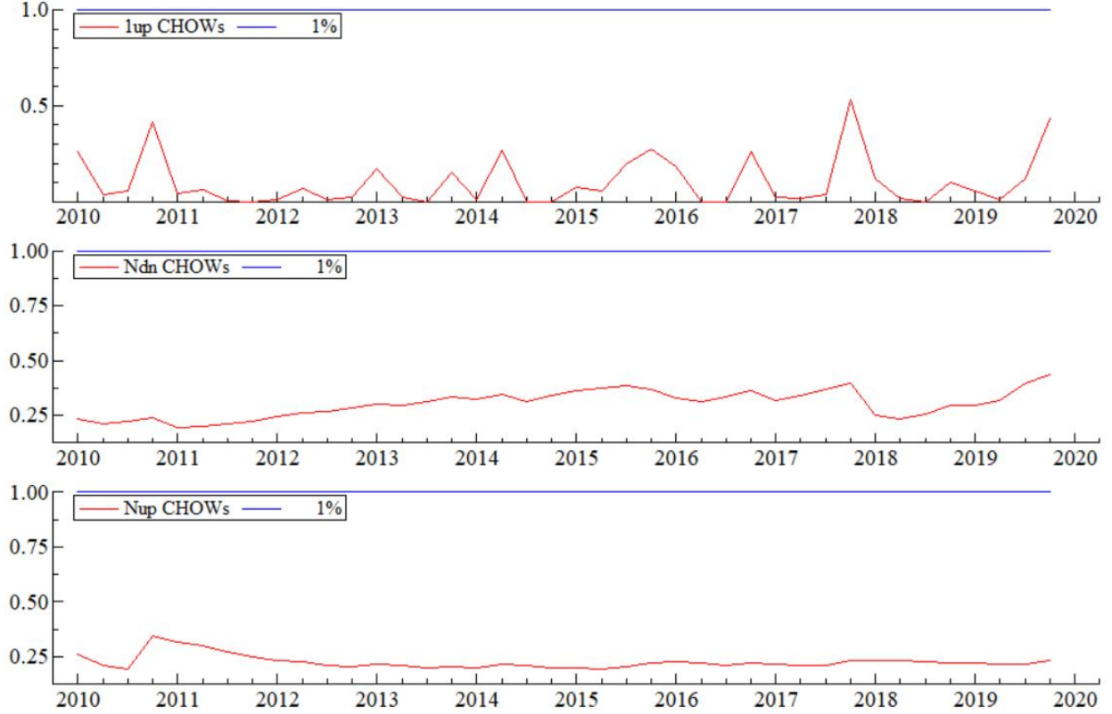
Figure 4: Stability Tests
