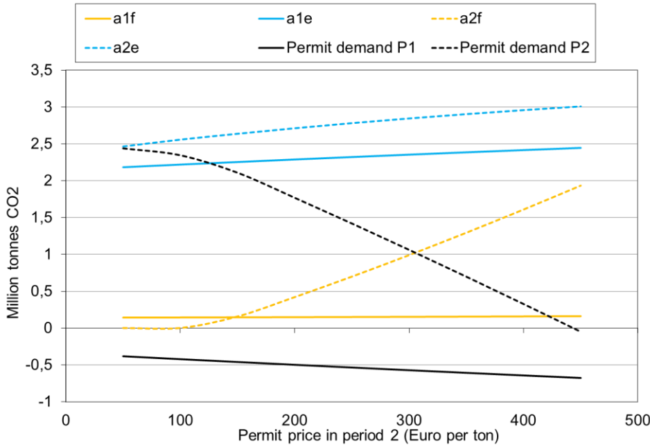
Figure 2: Effects of an increase in the permit price in Period 2 on the two abatement options and permit demand in a permit market with restrictions on banking and borrowing (spatial flexibility).
