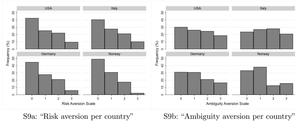
Figure S9: FREQUENCY OF RISK AND AMBIGUITY AVERSION SCALES BY COUNTRY
