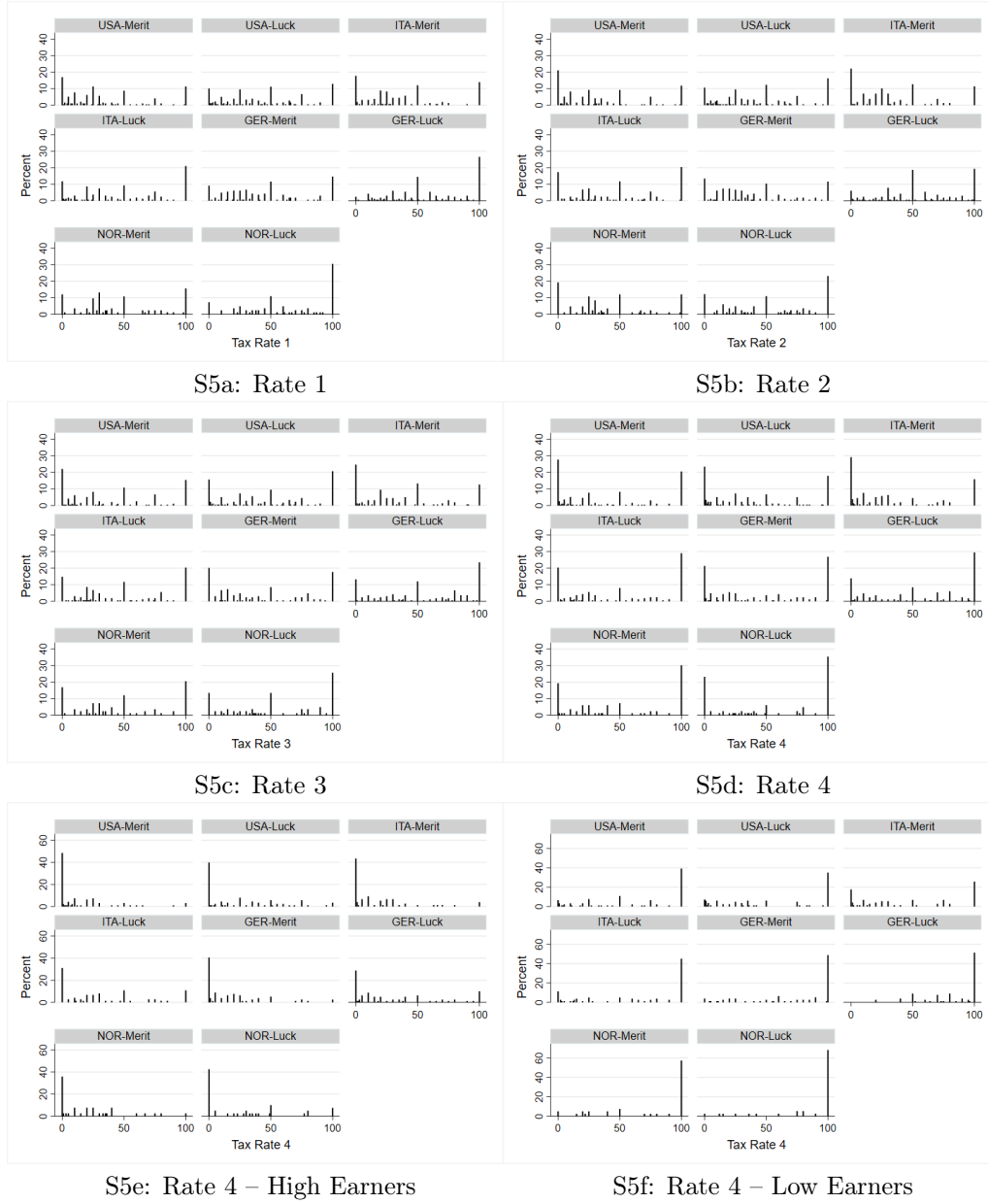
Figure S5: HISTOGRAMS OF REDISTRIBUTION DECISIONS BY COUNTRY
