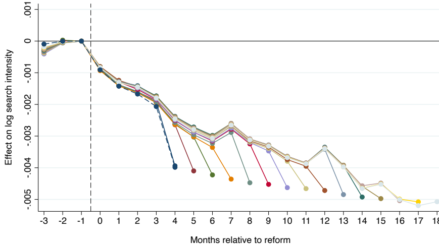
Figure 5: Varying the Effect Window (Crisis Sample)
