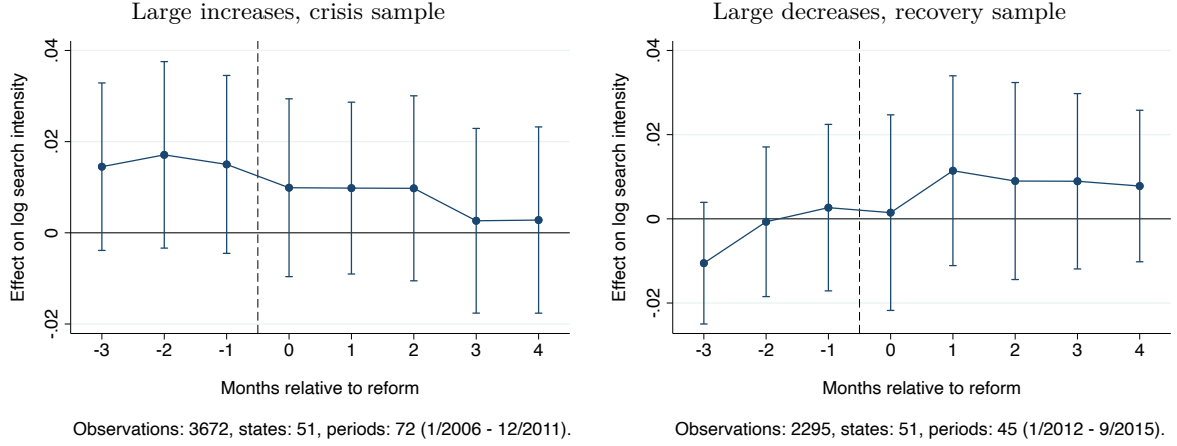
Figure 3: Baseline Results and the Role of Binning
