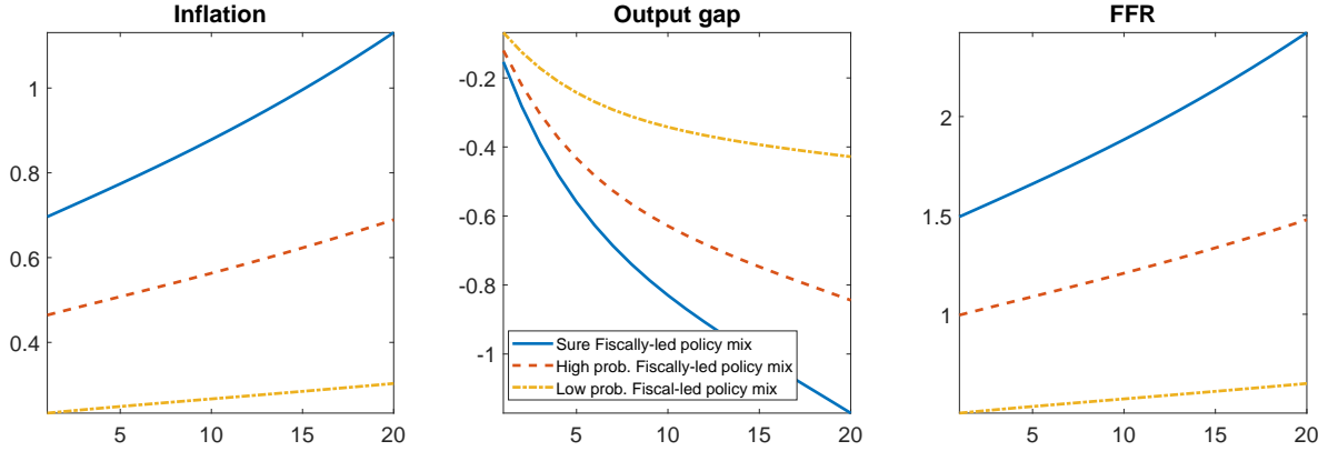
Figure 6 – Fiscal stagflation as agents’ beliefs about the future policy mix vary. Impulse responses of inflation, the output gap, and the federal funds rate (FFR) to a shock to long-term transfers as beliefs about the future policy mix change. The central bank responds to inflation as implied by the Monetary-led policy mix while the fiscal authority does not adjust taxes. The different lines correspond to different probabilities that the next policy mix will be Fiscally-led; – the blue line: Fiscally-led policy mix is expected to follow with certainty; orange dashed line: Fiscally-led policy mix is expected to follow with probability 0.67; yellow dotted-dashed line: Fiscally-led policy mix is expected to follow with probability 0.33.
