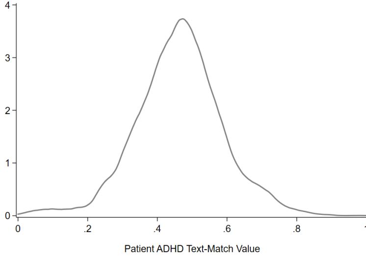
Figure 2: Density of ADHD Symptom Match x_i^*
