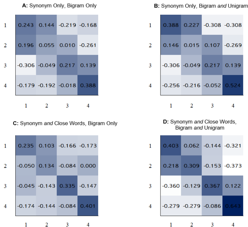
Figure 1: NLP Algorithm Correlation Plots
